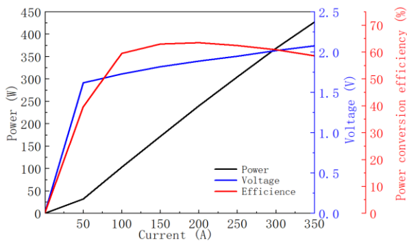
⊗ Power-Current-Voltage-Efficiency
